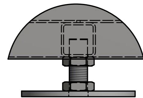
DETAIL B SCALE 1 / 2 ADJUSTABLE FEET
